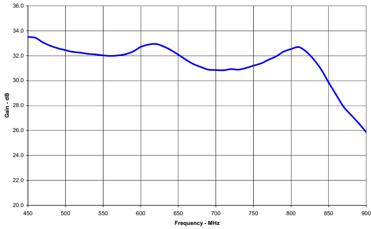
Gain vs. Frequency 28V DC 5W CW
