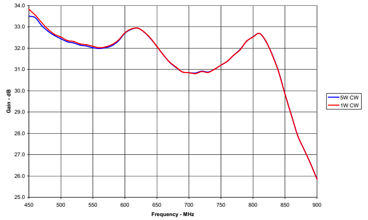
Effect of Power on Gain +28V DC
