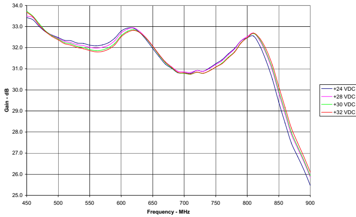
Effect of V supply on Gain at 5W CW
